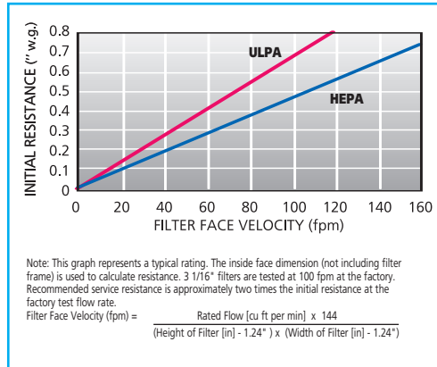
INITIAL RESISTANCE VS. FACE VELOCITY 2.5" MEDIA PACK
