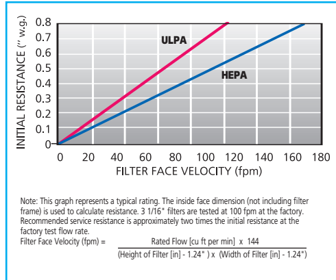
INITIAL RESISTANCE VS. FACE VELOCITY 2.5" MEDIA PACK
